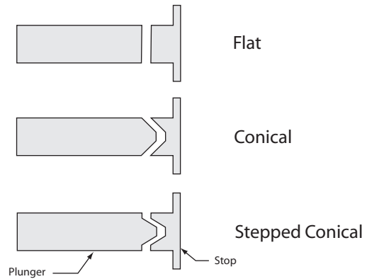
Figure 8 – Cross-sectioned, comparative views of flat, conical, and stepped conical stops and plungers, in a close to seated position.
